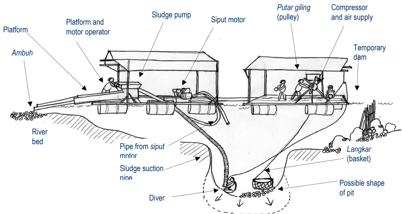
Picture 2 : Wet Suck Technology
